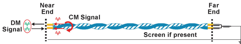
Figure 9: Typical transmission parameters for twisted pair cabling.
